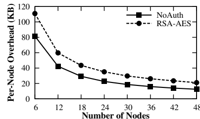
Figure 12: Per node communication overhead for secure hash join.
